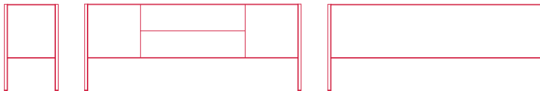
low unit 2 doors and double drawer L200 D50 H80 real dimensions L199.5 D50 H79.7 (L78-1/2" D19-3/4" H31-3/8")
