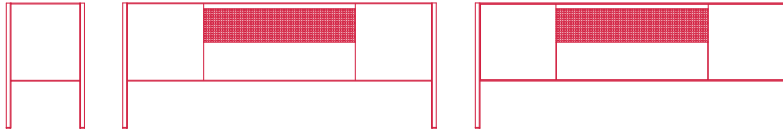
low unit 2 doors, single drawer and an open compartment L200 D50 H80 real dimensions L199.5 D50 H79.7 (L78-1/2" D19-3/4" H31-3/8")
