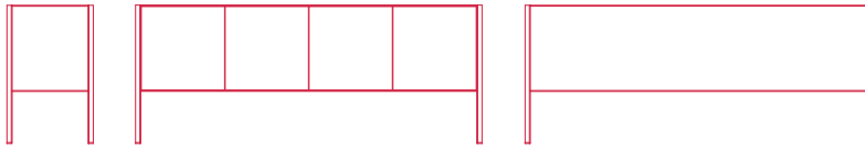
low unit 4 DOORS L200 D50 H80 real dimensions L199.5 D50 H79.7 (L78-1/2" D19-3/4" H31-3/8")
