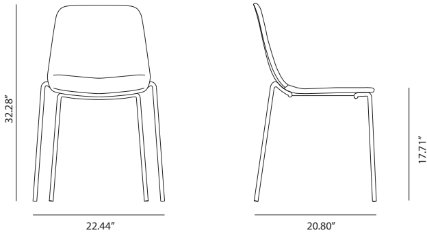
FOUR LEG BASE SMOOTH UPHOLSTERY
