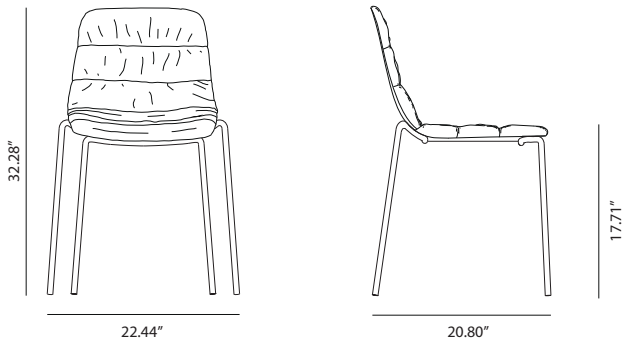
FOUR LEG BASE SOFT UPHOLSTERY
